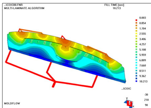
INJECTION PARE-CHOC
